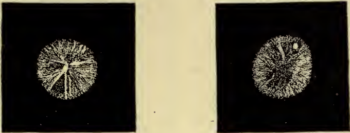
FIG. 47.—Two entoptic spectra in eyes which have perfect vision. These were seen when the person looked at the sky through a smooth stenopaic opening half a millimeter in diameter (Hess).
